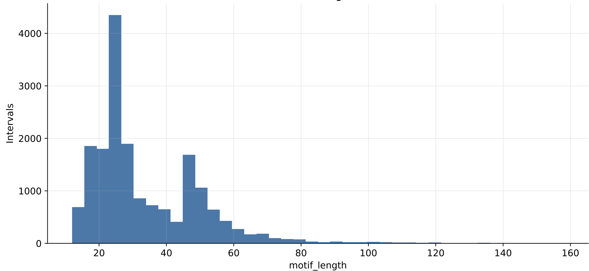
LoCoMotif interval length distribution
